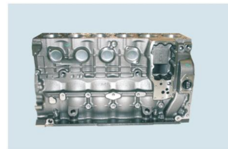
Cylinder Block ISB5.9(Bore 102mm) TPEC-ISB5.9缸体 (缸径102)
