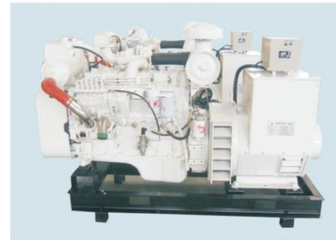
TPEC-Marine Generator Set
