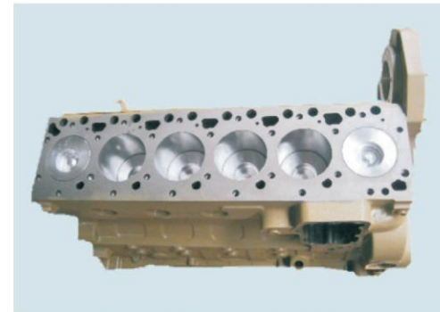
Short Block 4B/6B TPEC-4B/6B短缸体
