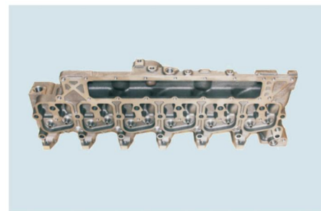
Cylinder Head 6B5.9 TPEC-6B5.9缸盖 3917287
