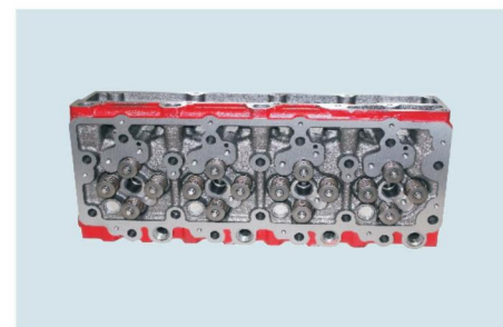
Cyl Head Assy ISF3.8 TPEC-ISF3.8缸盖总成 5258274V
