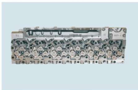
Cylinder Head Assy ISLe8.9L TPEC-ISLe缸盖总成 4942139
