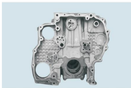
Cylinder Block OM471 TPEC-OM471 缸体
