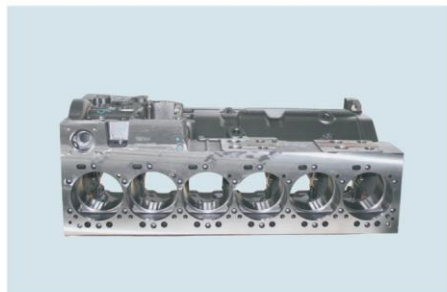
Cyl Block 6C New Type 5587414 TPEC-6C单节温新款缸体 5587414
