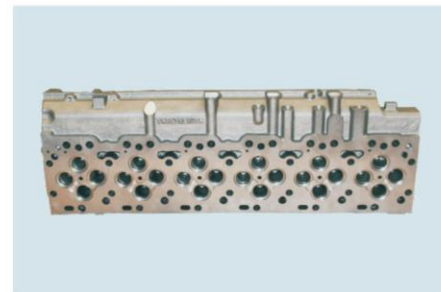
Cylinder Head QSC TPEC-QSC缸盖
