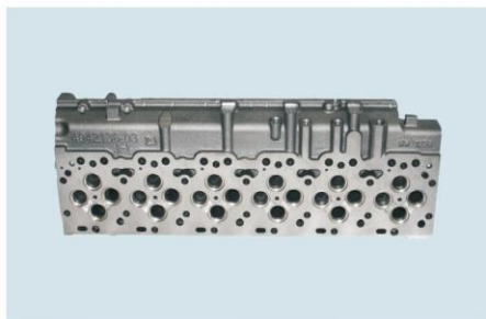
Cylinder Head ISLe8.9L TPEC-ISLe缸盖 4942138
