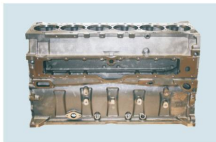
Cylinder Block X15 TPEC-X15缸体 4376170
